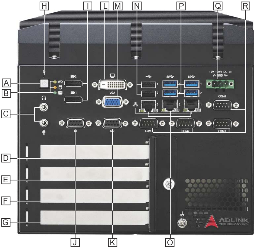
Figure 1-8: Front Panel I/O Connectors
