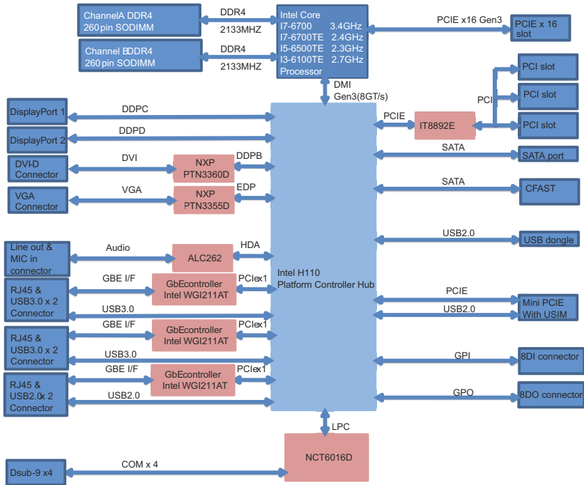
Figure 1-1: MVP-6010 Series Functional Block Diagram
