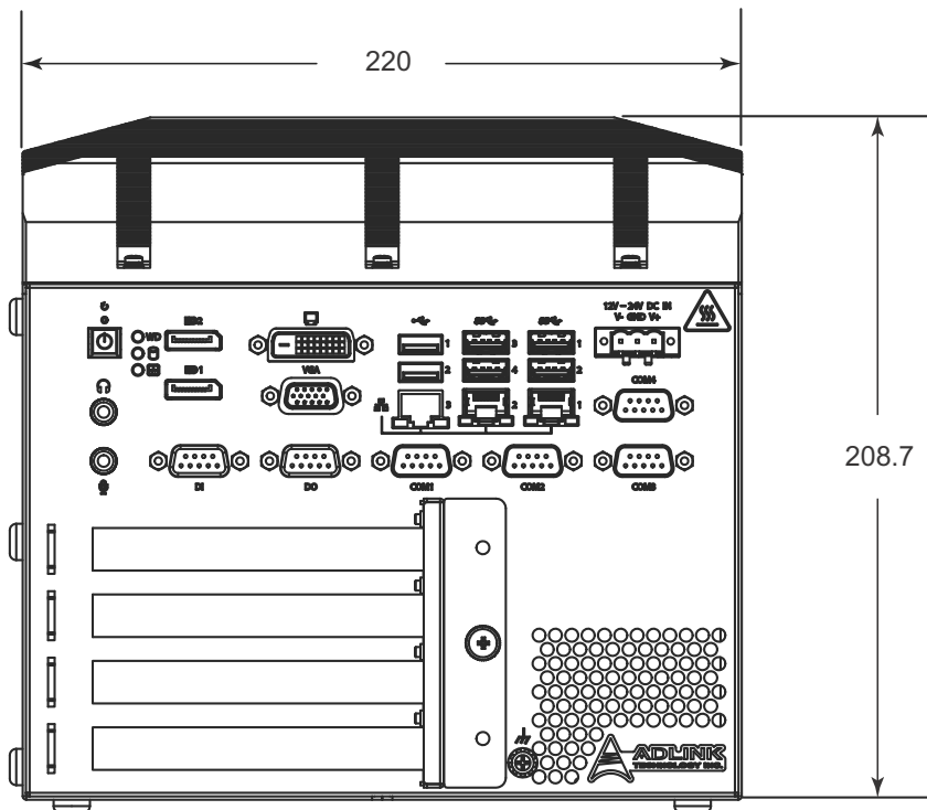
Figure 1-3: Front View
