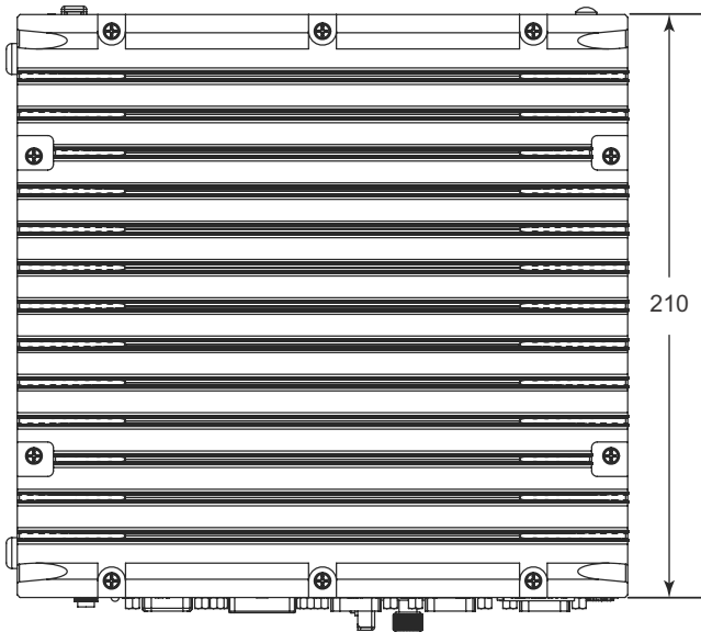
Figure 1-5: Top View
