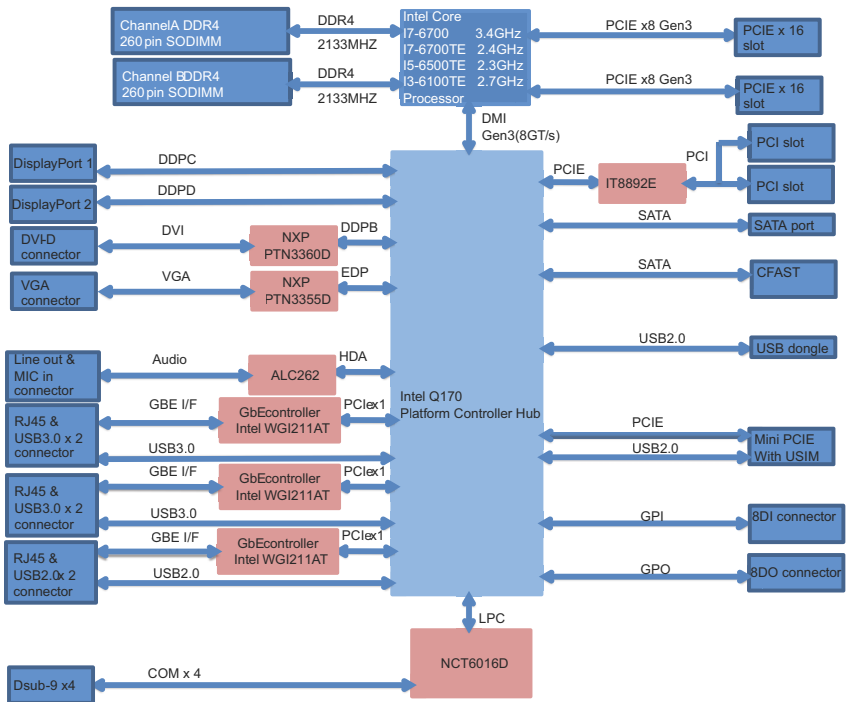
Figure 1-2: MVP-6020 Series Functional Block Diagram
