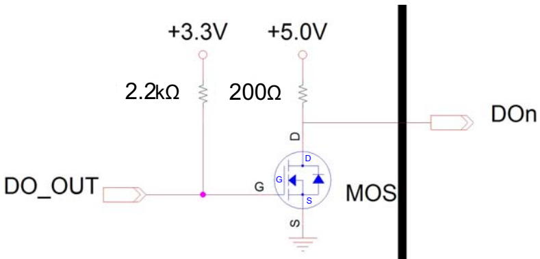
Figure 1-12: Digital Output Circuit
