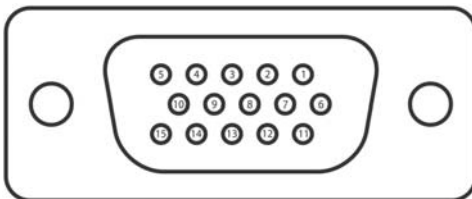
Figure 1-14: VGA Connector Pin Assignment
