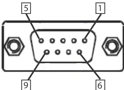
Figure 1-10: Digital I/O Connector Pin Assignment
