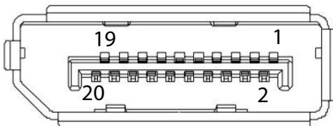
Figure 1-9: DisplayPort Connector
