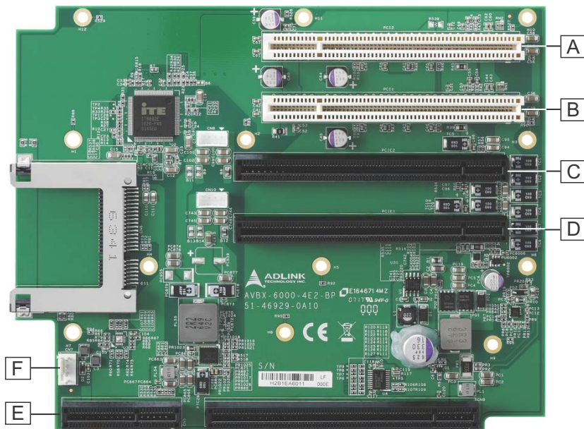
Figure 1-21: MVP-6020 Series Backplane Board PCB
