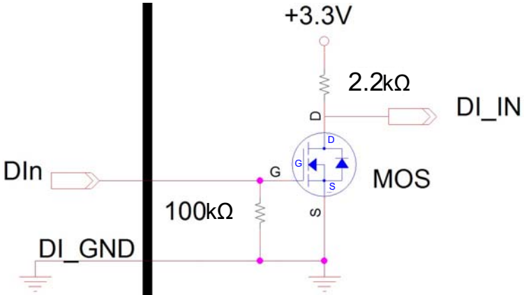
Figure 1-11: Digital Input Circuit
