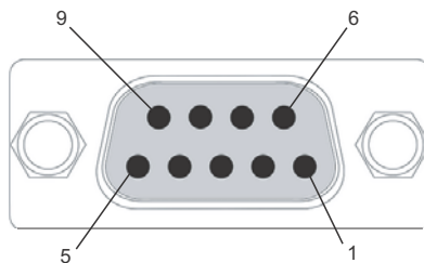
Figure 1-17: COM Port
