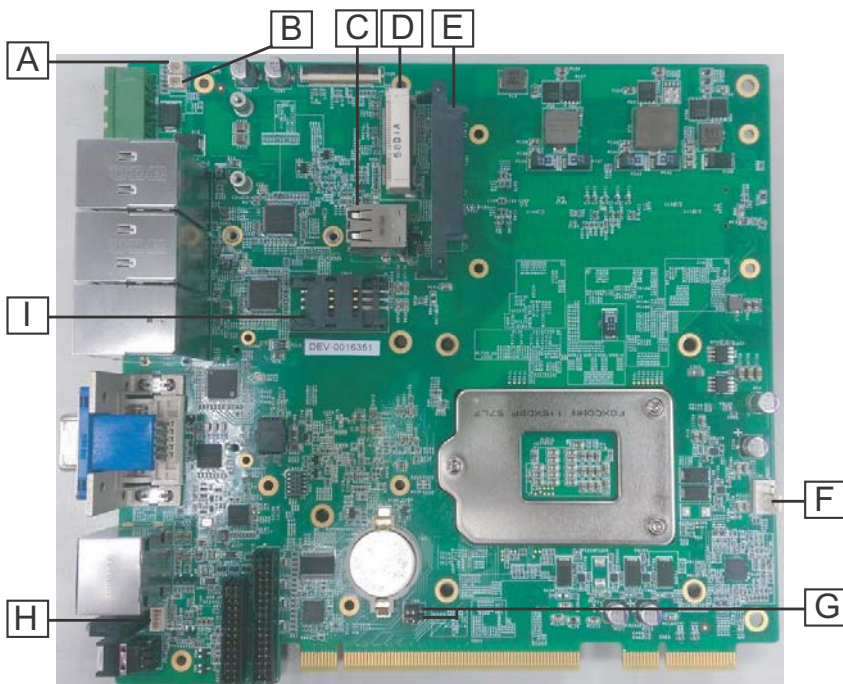
Figure 1-19: Mainboard I/O Connectors
