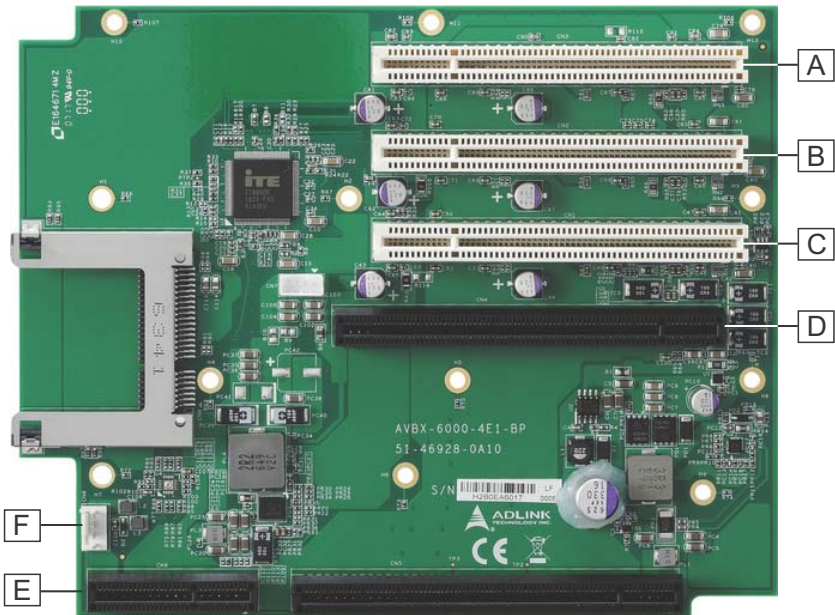
Figure 1-20: MVP-6010 Series Backplane Board PCB
